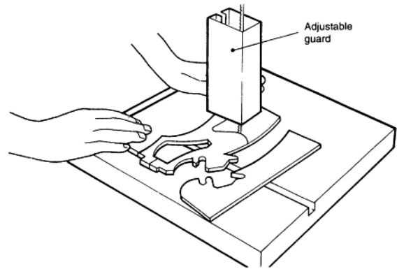
Figure 4 Freehand cutting
