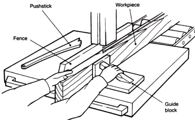
Figure 2 Straight cutting
